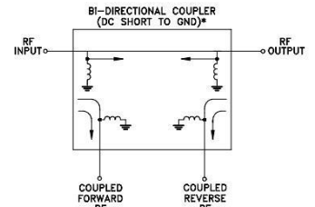
Electrical Schematic
